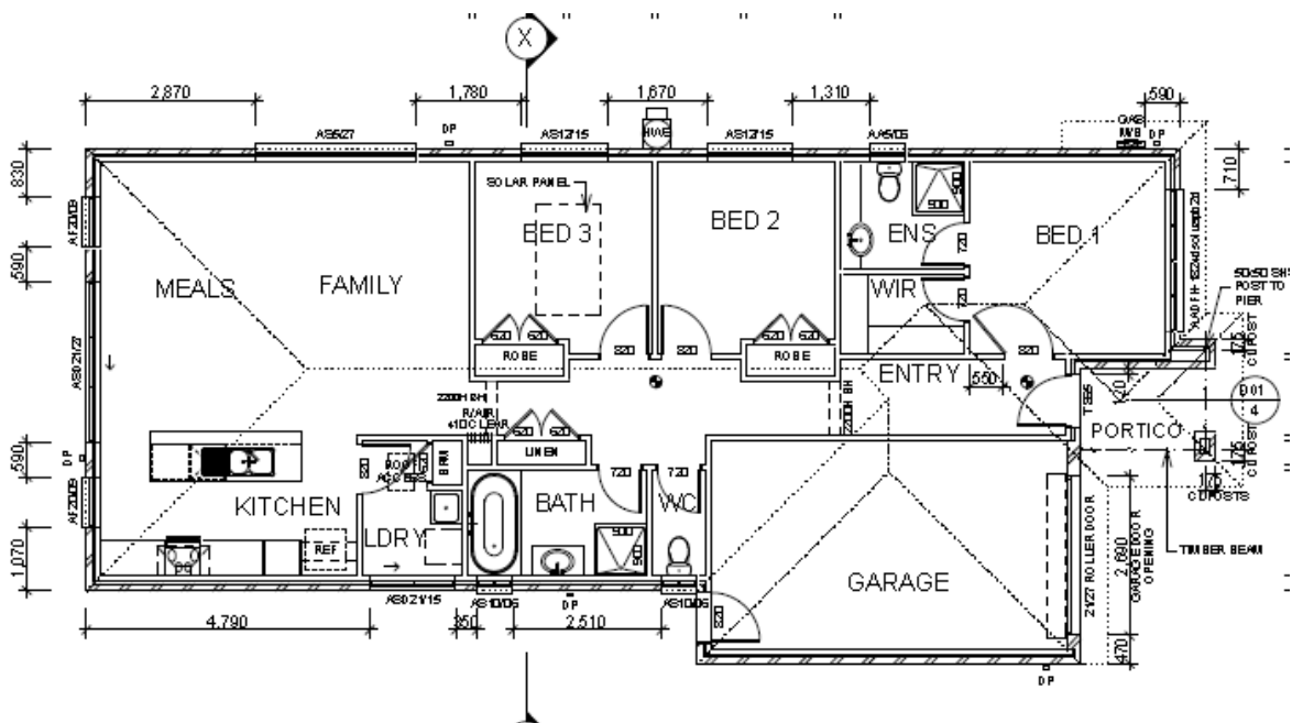
Floor Plan
