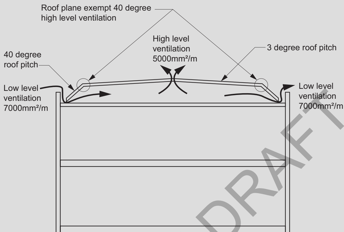
Figure F8D5c (explanatory):: Example of a multi-pitched roof space
