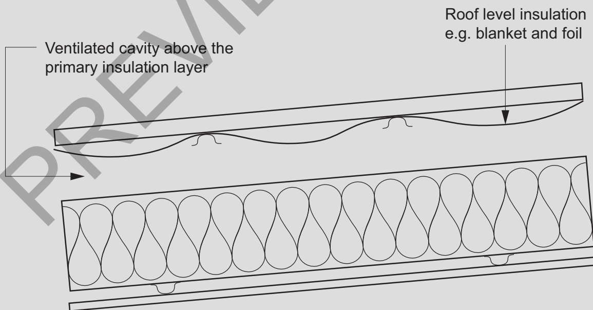
Figure Figure F8D6(b) (explanatory): Example of a roof space in accordance with F8D6(1)(a)(i)
