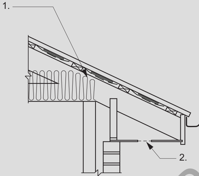
Figure F8D5a (explanatory): Example of roof space with low level of ventilation
