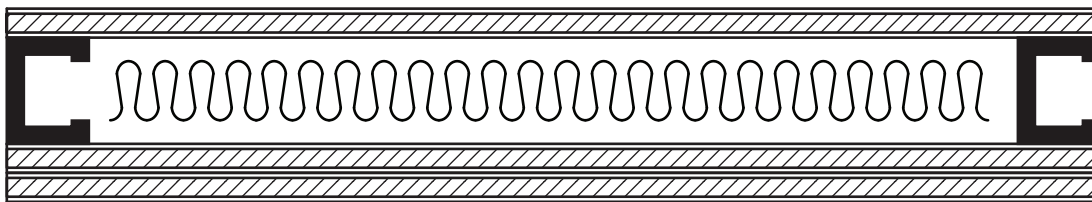
Figure S28C7j: One row of 64 mm steel studs with two layers of 13 mm plasterboard on each face
