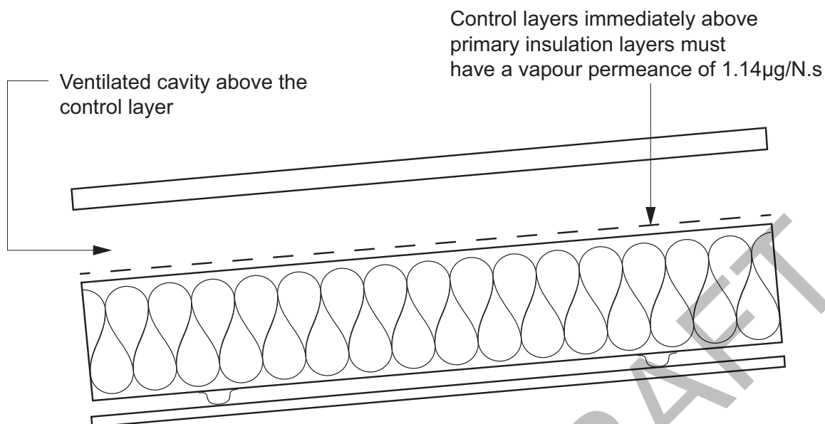
Figure F8D6c (explanatory): Example of a roof space in accordance with F8D6(1)(a)(ii)
