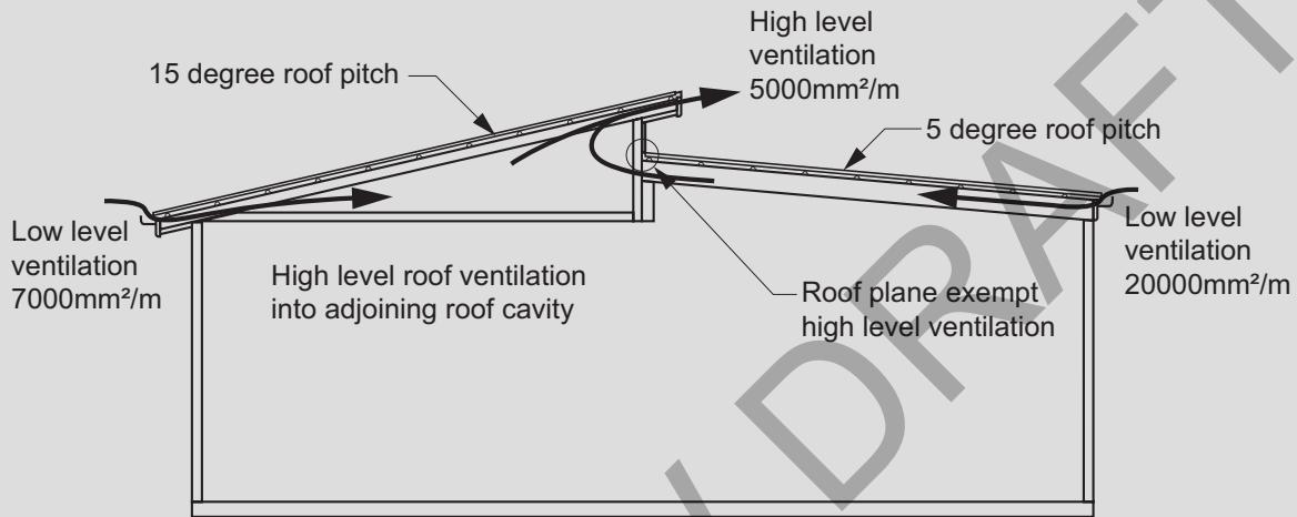
Figure F8D6a (explanatory): Practical example of a roof space with multiple roof types and requirements
